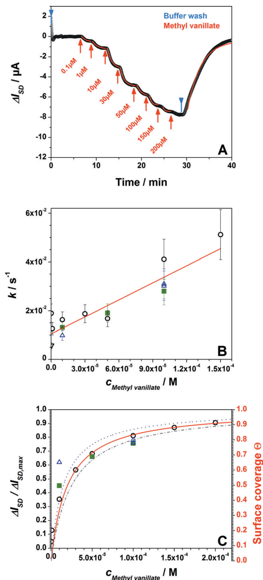
Figure 2. A) Real-time biosensor measurement of the binding of methyl vanillate to OBP14: the current increases with the bulk concentration of methyl vanillate increasing (from 100 nM to 200 \mu M) and then saturates. Blue arrows indicate runs with pure buffer, red arrows indicate experiments with methyl vanillate solutions. Red curves are the fitting of the raw data by kinetic simulations of the association and dissociation processes based on the Langmuir model. (For the estimation of the error limits, see the Supporting Information). B) Analysis of the reaction rate constants, k , obtained from the fitted data in (A) as a function of methyl vanillate concentration; different symbols from three different devices; error bars are \pm 20\% . C) Langmuir adsorption isotherm, obtained for three different samples; the red fit curve gives K_d = 20 \mu M (plotted are also error limits for K_d of 20%).
